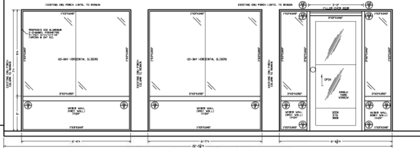
PROPOSED BACK ELEVATION [PARTIAL] SCALE OF 1/4" = 1'-0"
