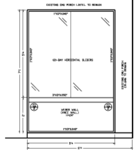
PROPOSED RIGHT ELEVATION [PARTIAL] SCALE OF 1/4" = 1'-0"
